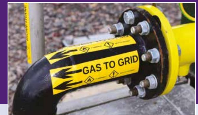
Upgraded methane is injected directly into the national gas grid
